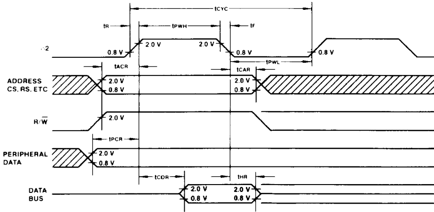
Figure 1. Read Timing
